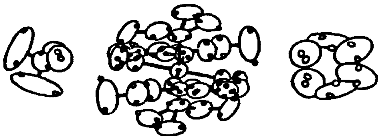
Fig. 1. The relationship between the room-temperature ( C2/c ) and the low-temperature ( P2_1/c ) structures. Thermal ellipsoids from the room-temperature structure are superimposed with small circles which indicate the atomic positions at low temperature and the low-temperature positions translated by (a+b)/2 . This figure suggests that the refined room-temperature thermal parameters mask a disorder of the two independent orientations observed at low temperature. (Reprinted with permission from ref. 40.)
